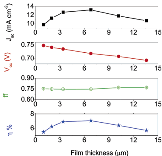
Figure 4. The detailed photovoltaic parameter ( J_{sc} , V_{oc} , FF, and \eta ) variations with different film thicknesses of transparent layer and keeping constant 4 \mu\text{m} reflecting layer based on K-19 dye, and PPA as coadsorbent and ionic liquid electrolyte.
