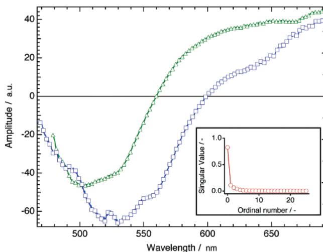
Figure 1. Base vector from the SVD of K19 observed on \text{TiO}_2 following excitation at 520 nm ( \square ) and on \text{Al}_2\text{O}_3 after excitation at 500 nm ( \Delta ). The inset shows the singular values of the decomposition for the data obtained on \text{TiO}_2 ( \circ ).
