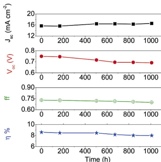
Figure 7. Photovoltaic parameter ( J_{sc} , V_{oc} , FF, and \eta ) variations with aging time for the device based on (6.8 + 4) \mu\text{m} film sensitized with K-73/DPA and nonvolatile electrolyte during successive one sun visible-light soaking at 60^\circ\text{C} .
